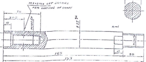
SHAFT (300 MCD. ALL OVER) MAT:- EN-39 QTY:- 1 No.
