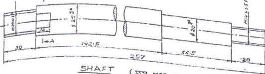
SHAFT (300 MCD. ALL OVER) MAT:- EN-39 QTY:- 1 No.
