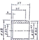
BUSH (200 MCD. ALL OVER) MAT:- EN-39 QTY:- 1 No.
