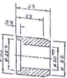
BUSH (300 MCD. ALL OVER) MAT:- EN-39 QTY:- 1 No.
