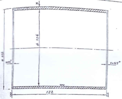
CYLINDER MAT:- STAINLESS STEEL (AISI-304) QTY:- 1 No.
