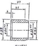
BUSH (SEE MCD. ALL OVER) MAT: - EN-39 QTY: - 1 No.
