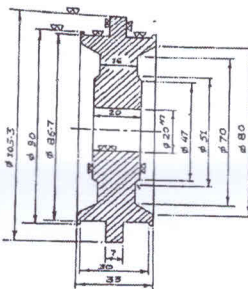
PISTON MAT: - CARBON STEEL (S:120305-30-40) QTY: - 1 No.
