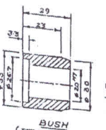
BUSH (SEE MCD. ALL OVER) MAT: - EN-39 QTY: - 1 No.
