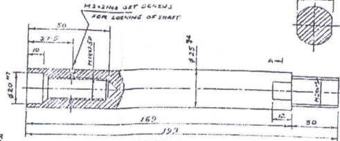
SHAFT (SEE MCD. ALL OVER) A-A MAT: - EN-39 QTY: - 2 No.
