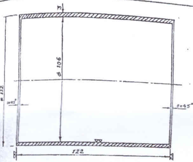
CYLINDER MAT: - STAINLESS STEEL (AISI-304) QTY: - 1 No.
