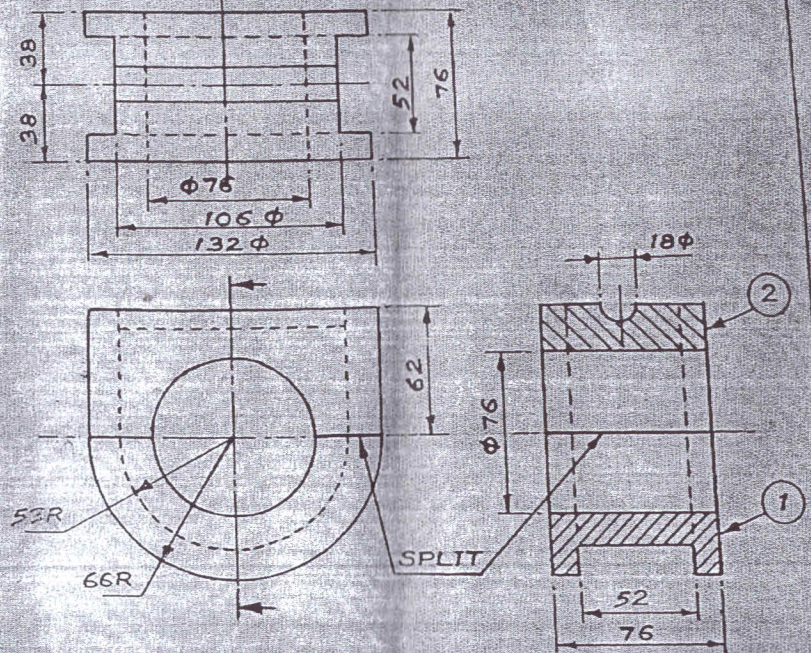
HANGER BEARING IN TWO PARTS (SPLIT) (▽ MACHINED ALL OVER) MAT.:- CAST IRON (IS:210 Gr.FG-220)
