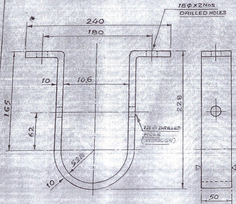
HANGER FOR BEARING MAT. - M.S.
